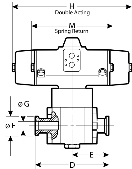
Actuator Operator with G-CON Hub End Connection
